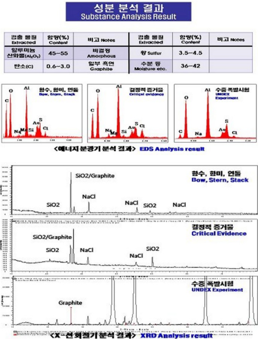
Figure 4. JIG's EDS and XRD
